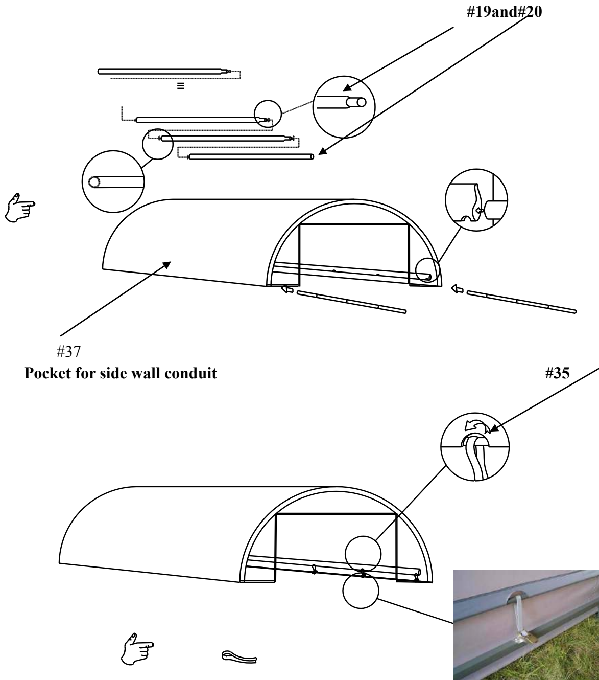
Ratchet Tie-Down for Tensioning the side wall (roof cover)
